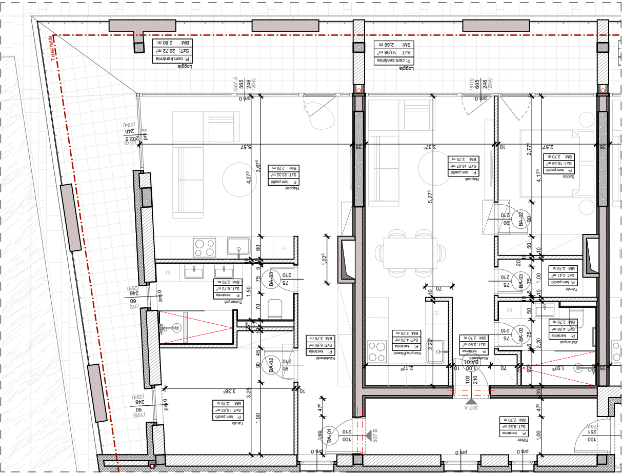
III. emelet - 307/A Lakás
